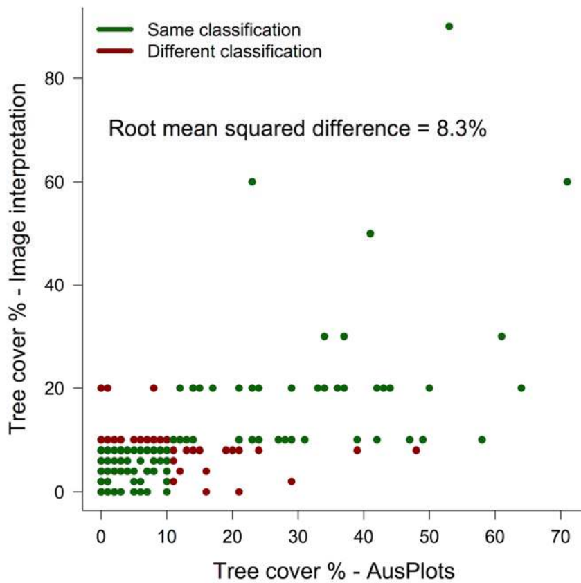
Fig. 4. Application of TERN AusPlots data to an accuracy assessment for tree cover estimates and forest classification from 'CollectEarth' (Very High Resolution satellite image interpretation) as part of the Global Drylands Assessment of the United Nations FAO. Bastin et al. (2017) reported an increase in known forest stands in global drylands of 40-47%, with field validation and assessment of uncertainty from AusPlots.
