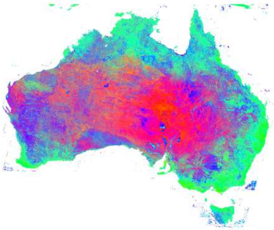
Figure 4. Example of a Landsat fractional cover mosaic for Australia. Green vegetation is shown in green, non-green cover is blue and bare ground is red. These data are publicly available from TERN's Auscover facility
